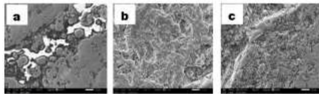
Figure 6. Microstructure with annealing variation at temperature a. 800 °C, b. 900 °C dan c. 1000 °C
