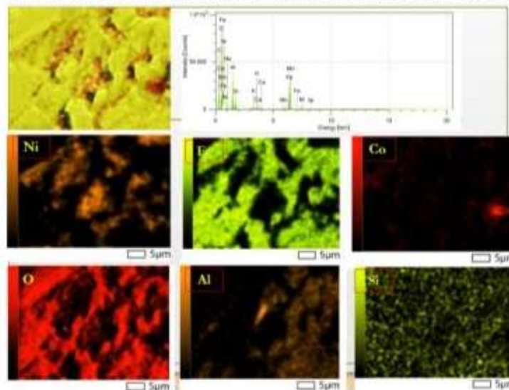
Figure 8. EDS mapping on Fe-Ni-Co alloy after 900 °C annealing
