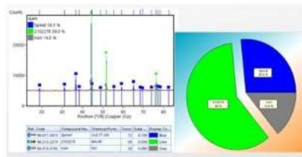
Figure 2. Detailed analysis of XRD-spectra at 4 hours milling
