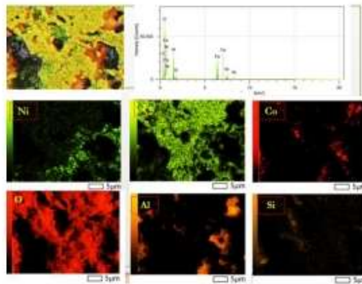
Figure 9. EDS mapping on Fe-Ni-Cu alloy after 1000 °C annealing
