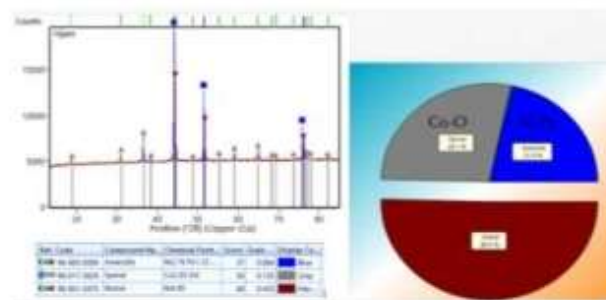
Figure 4. Detailed analysis of XRD-spectra at 16 hours milling
