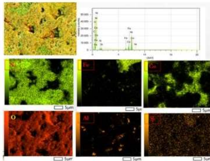
Figure 7. EDS mapping on Fe-Ni-Co alloys after 800 °C annealing.
