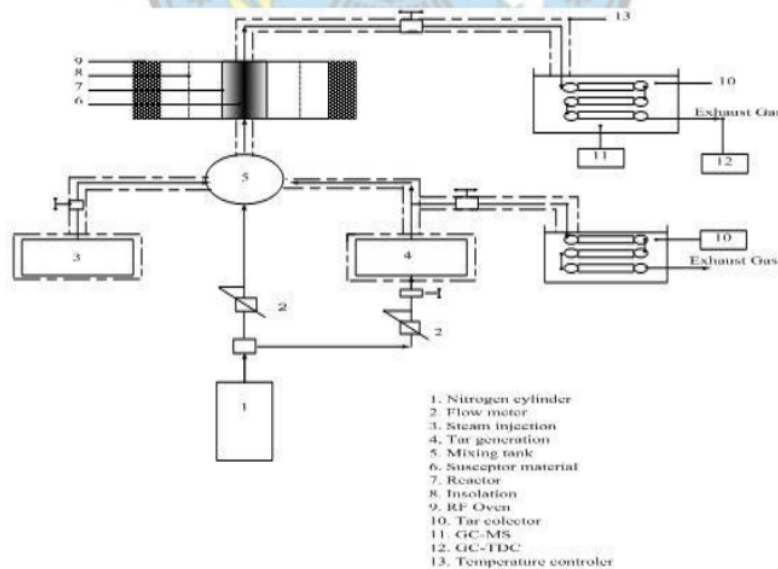
Gambar 2. Sketsa diagram peralatan percobaan
