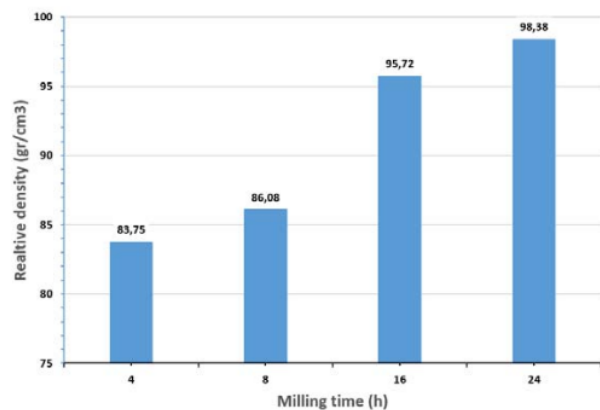
Figure 6. Relative density of the TiTaVWCr
