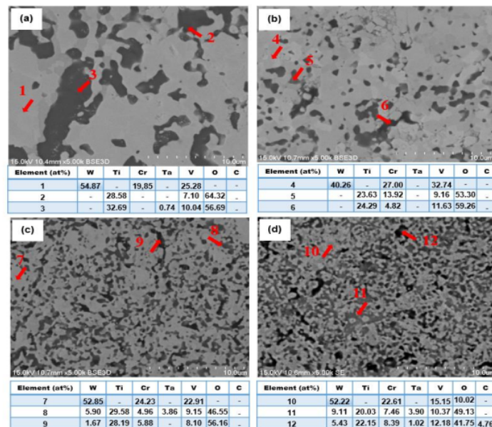
Figure 3. EDS images of the TiTaVWCr at grinding time of (a). 4 h, (b). 8 h, (c). 16 h and (d). 24 h
