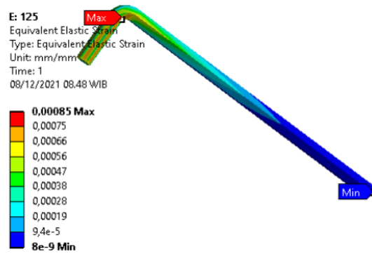
Gambar 10. Hasil Equivalent Elastic Strain Simulasi Pembebanan 125 N
