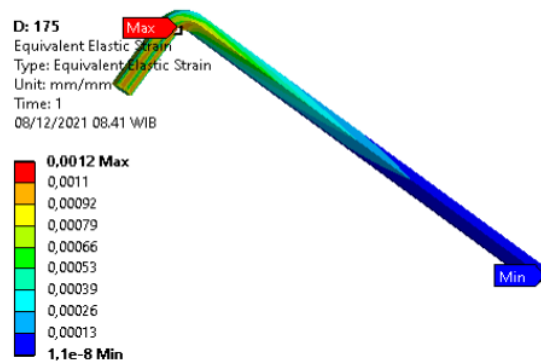
Gambar 11. Hasil Equivalent Elastic Strain Simulasi Pembebanan 175 N
