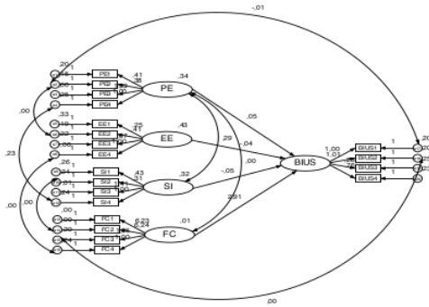
Gambar 4. Full Model Struktural
