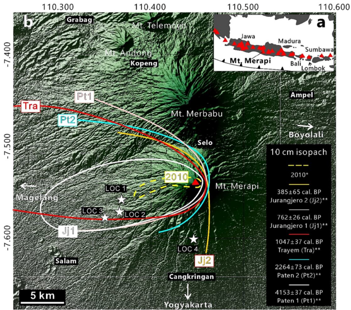
Fig. 1. (a) A sketch map showing the location of Merapi volcano in Central Java, Java Island. Red triangles are active volcanoes, while grey area represent 5 lands. Black solid line with triangles is the subduction zone between Indo-Australia and Eurasia. (b) 10-cm isopach of some VEI 3–4 eruptions of Merapi volcano (Paten I, Paten II, Trayem, Jurangjero I, Jurangjero II, and 2010 CE) obtained from Gertisser et al., 2012 and Solikhin et al., 2015. Our sampling locations were focused on the western flanks because, all of those fall deposits were distributed to west side (towards Magelang City). We visited the southern flank with aim to sample an unnamed Young Merapi pumice fall deposit (~20–30 cm 18 k) as reported in Gertisser et al. (2011; see their Fig. 7c). Digital elevation model image was obtained from Badan Informasi Geospasial (BIG) Indonesia 2022. (For interpretation of the references to colour in this figure legend, the reader is referred to the web version of this article.)
