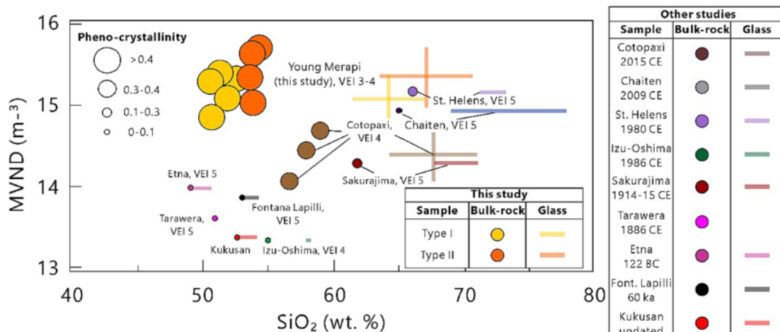
Fig. 14. Comparison of MVND and \text{SiO}_2 plot between the Young Merapi pumices (this study, shown by yellow and orange circles) with juveniles from the other sub-Plinian/Plinian eruptions. Note that each circle size denotes different pheno-crystallinity value. Larger eruption (VEI 5) tend to be associated with less crystalline magma (30% pheno-crystallinity), while smaller eruptions (VEI 3–4) include more phenocrysts (up to >40%). (For interpretation of the references to colour in this figure legend, the reader is referred to the web version of this article.)
