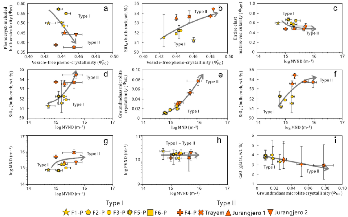
Fig. 11. Correlation of some important textural parameters. (a, b) Vesicle-free pheno-crystallinity ( \Phi_{PC}^v ) is found to be negatively and positively correlated with bulk-vesicularity ( \Phi_{BV} ) and bulk-rock silica content. (c, d) Matrix-vesicle number density (MVND) shows negative and positive correlation with matrix-vesicularity ( \Phi_{MV} ) and bulk-rock silica content. (e, f) Microlite number density (MND) is positively correlated with microlite fraction ( \Phi_{MC} ) and bulk-rock silica content. (g) Positive correlation between MVND and MND. (h) Constant correlation between MVND and PVND. (i) Negative correlation between \Phi_{MC} and CaO_{glass} .
