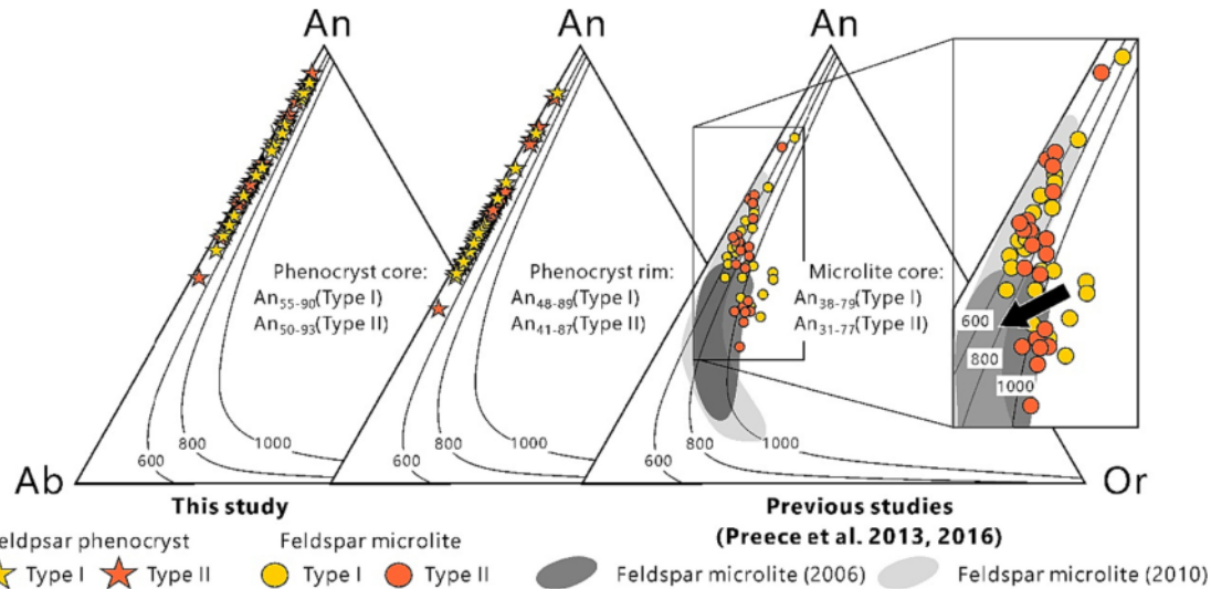
Fig. 8. Ternary feldspar diagram of Young Merapi pumice falls for feldspar phenocryst core (left), rim (middle), and feldspar microlite (right). Isothermal sections (i. e., magma temperature) of the dry ternary solvus was adapted from Preece et al., 2016, using VOLCALC (Wen and Nekvasil, 1994). Both pumice type shares relatively similar feldspar phenocryst core compositions ( An_{55-90} for type I and An_{50-93} for type II). However, note type I has slightly more calcic feldspar phenocryst rim ( An_{48-89} for type I and An_{41-87} for type II) and microlite ( An_{38-79} for type I and An_{31-77} for type II) compositions than type II.
