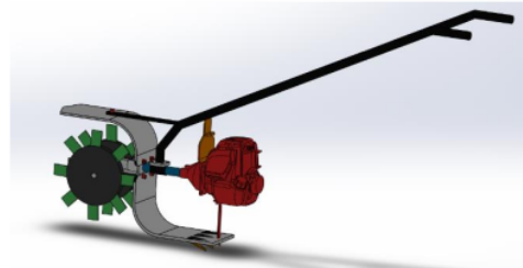
Figure 1. Design of weed weeding machine
