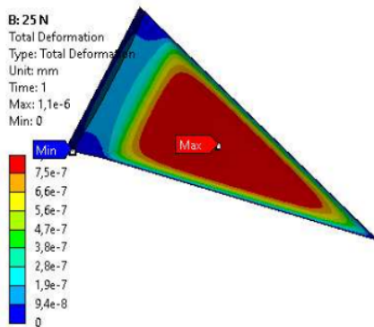
Figure 10. Deformation 25 N
