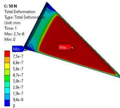
Figure 11. Deformation 50 N
