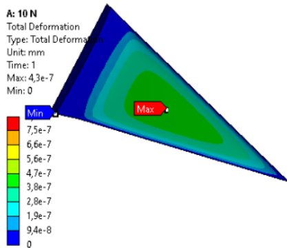
Figure 9. Deformation 10 N
