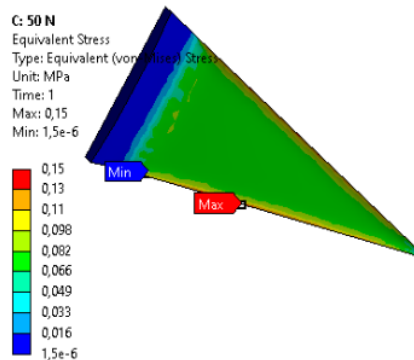
Figure 8. Von Mises Stress 50 N
