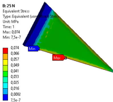
Figure 7. Von Mises Stress 25 N
