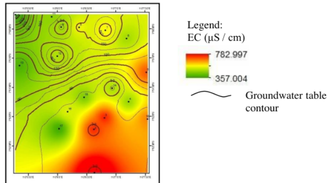
Figure 10. Iso-EC map of groundwater in research area.
