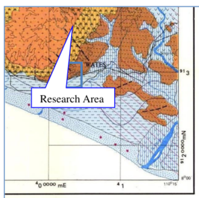
Figure 4. Research area in hydrogeological map [11].
