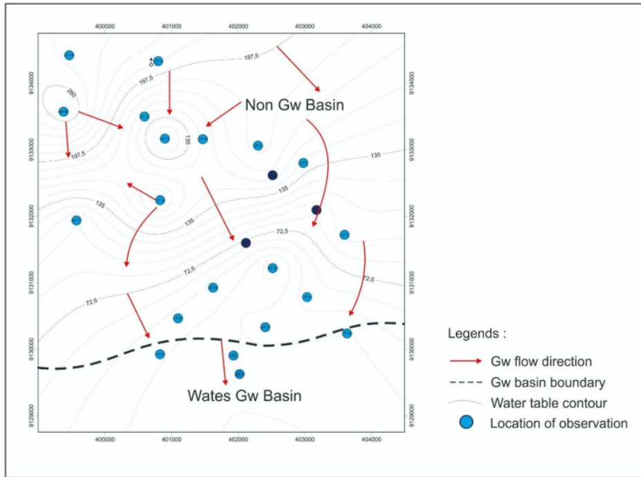
Figure 6. Groundwater table map of research area.
