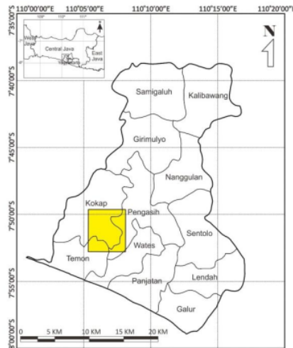
Figure 1. Location of research area.
