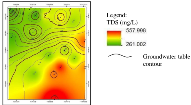
Figure 9. Iso-TDS map of groundwater in research area.
