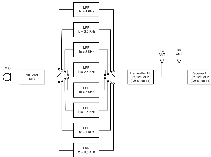
Gambar 4. Blok Diagram Penelitian
