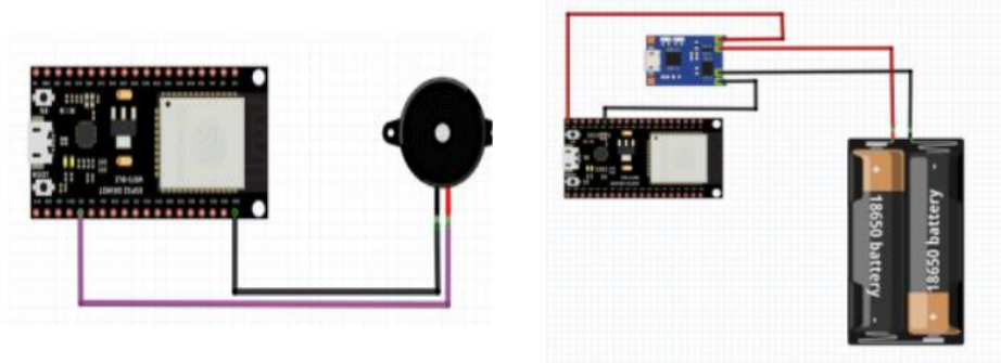
Rangkaian Buzzer
