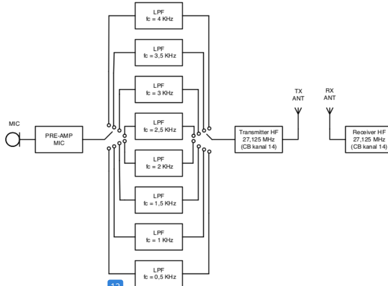
12 Gambar 4. Blok Diagram Penelitian
