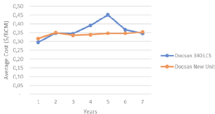
Gambar 2. Grafik Average Unit Cost Doosan 340 DX LC5
