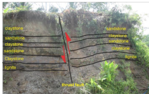
Figure 2. Sandstone and claystone interbedded with lignite intercalation
