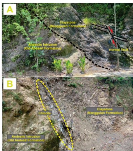
Figure 3. A. An Andesite Dike Old Andesite Formation intrudes sedimentary rock (Nanggulan Formation) at Sermo (SRM-2). B. Chlorite as a characteristic of the metamorphism process caused by the andesite dike at Sermo (SRM-2).
