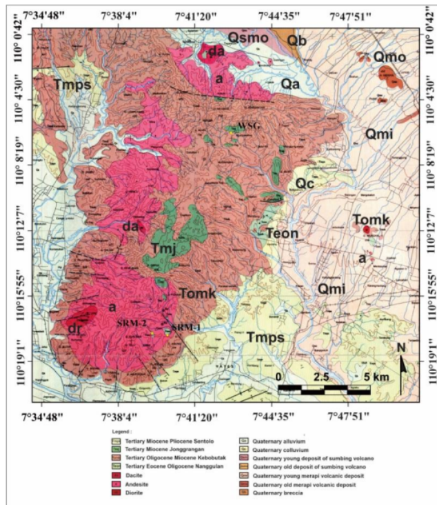
Figure 1. Samigaluh (WSG) and Sermo (SRM-2) are located in the central Kulon Progo Mountains, which are part of the Kebobotak Formation (Tomk) and Andesite (a).
