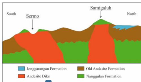
Figure 7. Model of the Nanggulan Formation roof pendant on the central side of Kulon Progo
