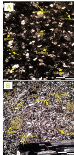
Figure 4. Petrographic analysis results at Sermo-2 (cross-polarized light position). A. Sandstone indicated the existence of pyrite and kaolinite, which indicate hydrothermal alteration. B. Chlorite minerals indicate andesite dike as evidence of hydrothermal alteration.
