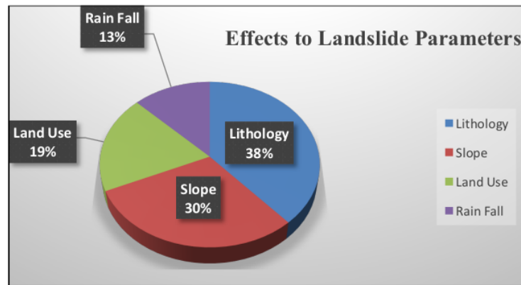
Figure 5. Distribution of Effect for Landslide Parameters
