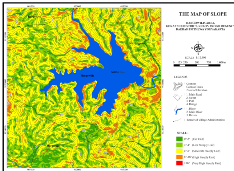
Figure 1. The slope map in research are
