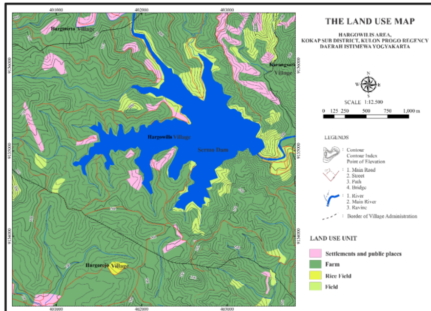
Figure 3. The land use map in research area
