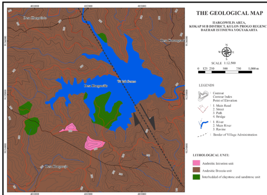
1 Figure 2. The geological map in research area shows the distribution of rocks Mapping of Landslide Susceptibility based on AHP in Sermo dam and its surrounding, Kokap, Kulon Progo (Al Hussein Flowers Rizqi et al)
