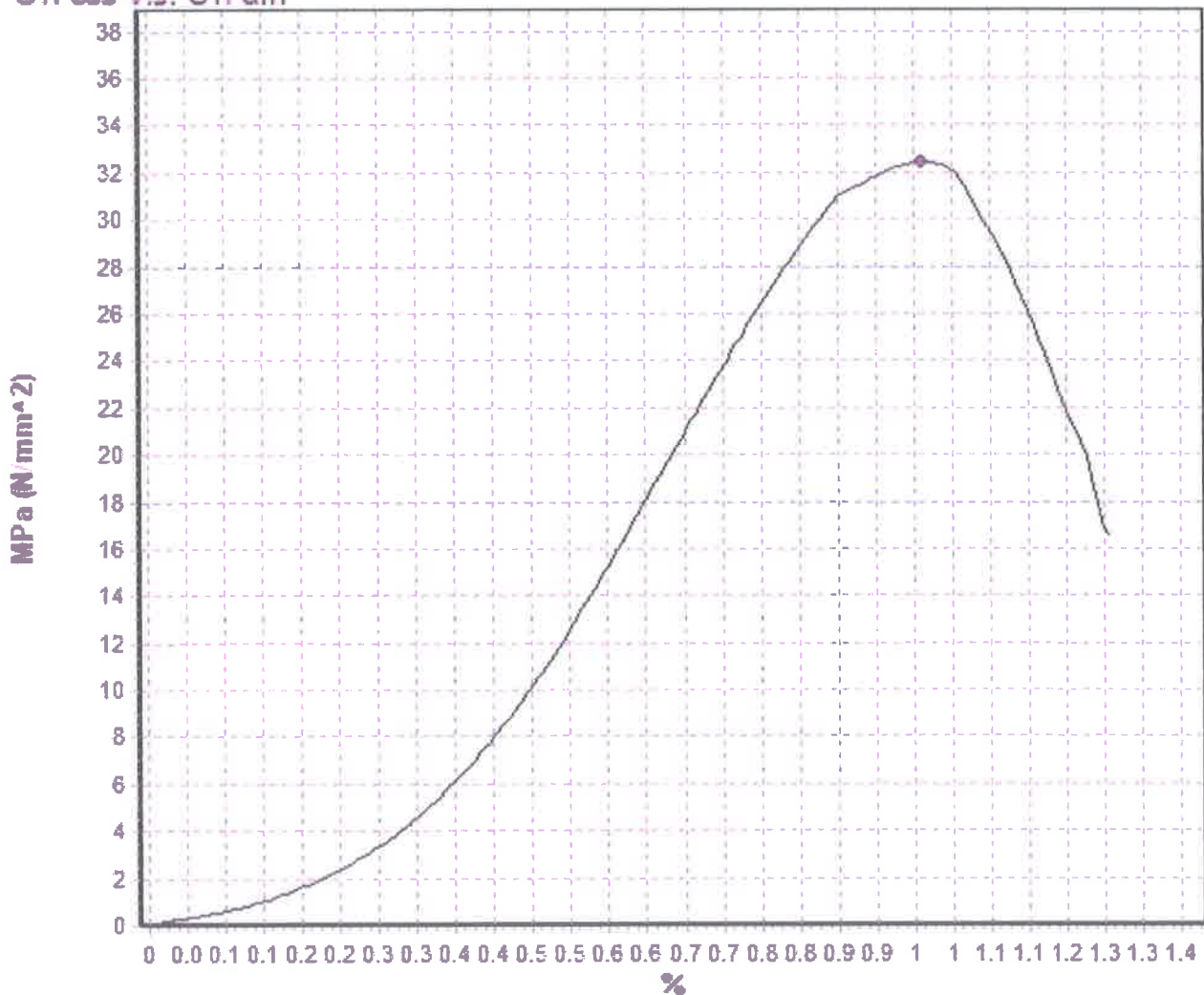
Stress v.s. Strain
