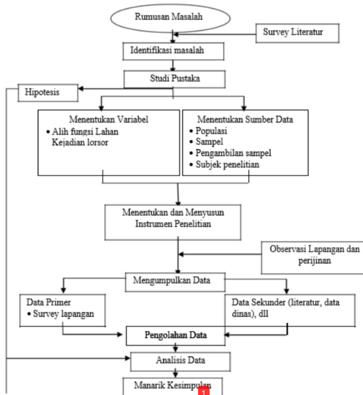
Gambar 2. Alur penelitian
