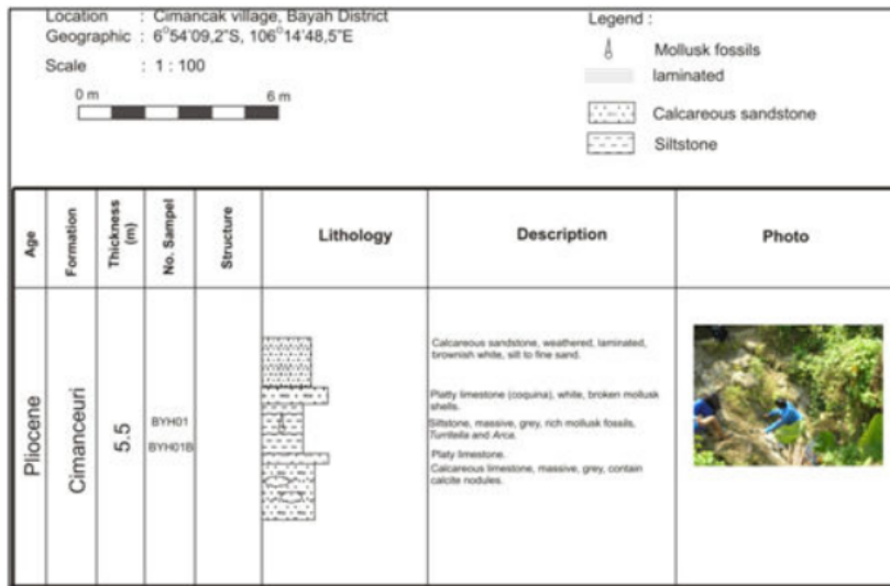
Figure 2. Outcrop profile of Bayah site
