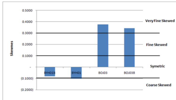
Figure 8. Skewness value from four samples, show BOJ samples are very fine and BYH symetrical skewness
