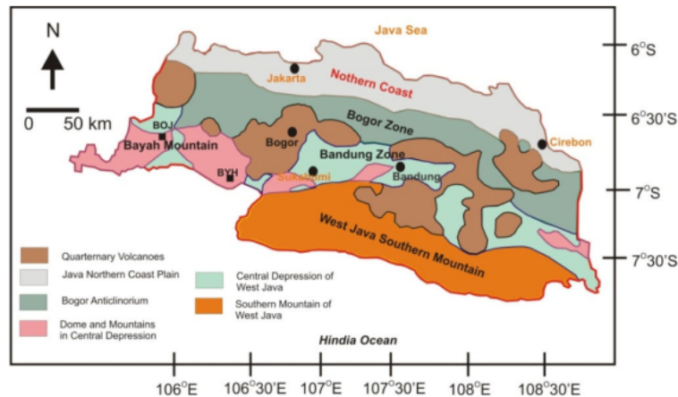
Figure 1. West Java physiography (redrawn from van Bemmelen, 1949) and the study area at Bojong (BOJ) and Bayah (BYH).
