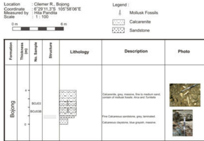
Figure 3. Outcrop profile of Bojong site
