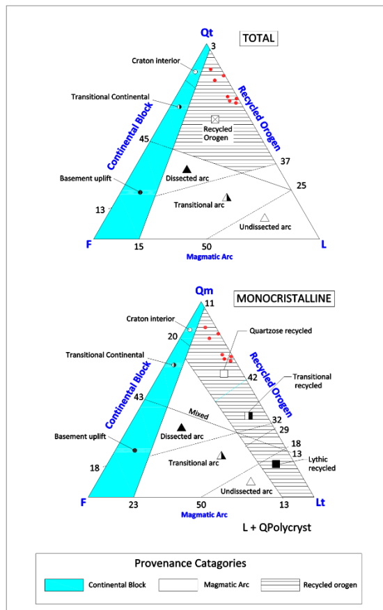
Fig.3 Provenance classification of Warukin sandstones
