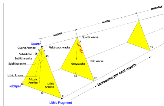
Fig.2 Classification of Warukin sandstones according to the classification by Pettijohn 1975.
