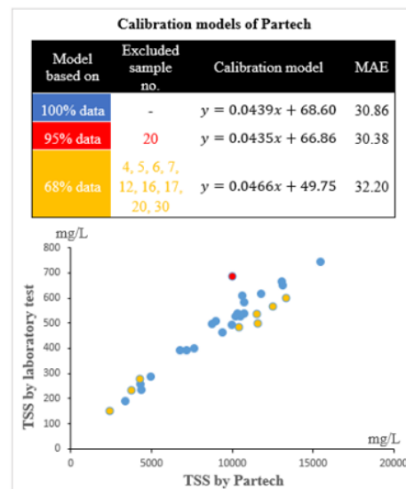
Fig.4 Plot of TSS value by laboratory test against TSS value by Partech 740 as well as the excluded TSS value points on model 95% (red) and 68% (yellow)
