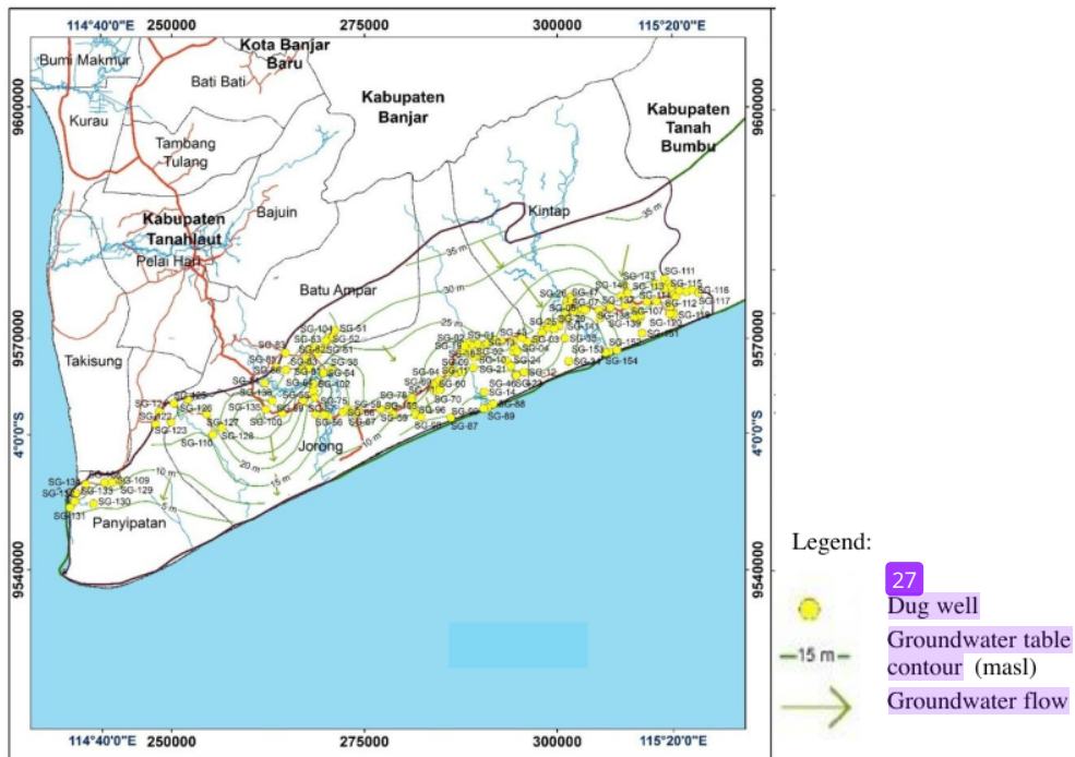
Figure 3. Shallow groundwater table map of research area.
