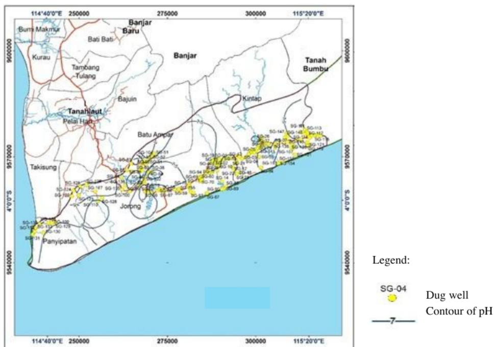
Figure 5. The distribution of pH in free groundwater.
