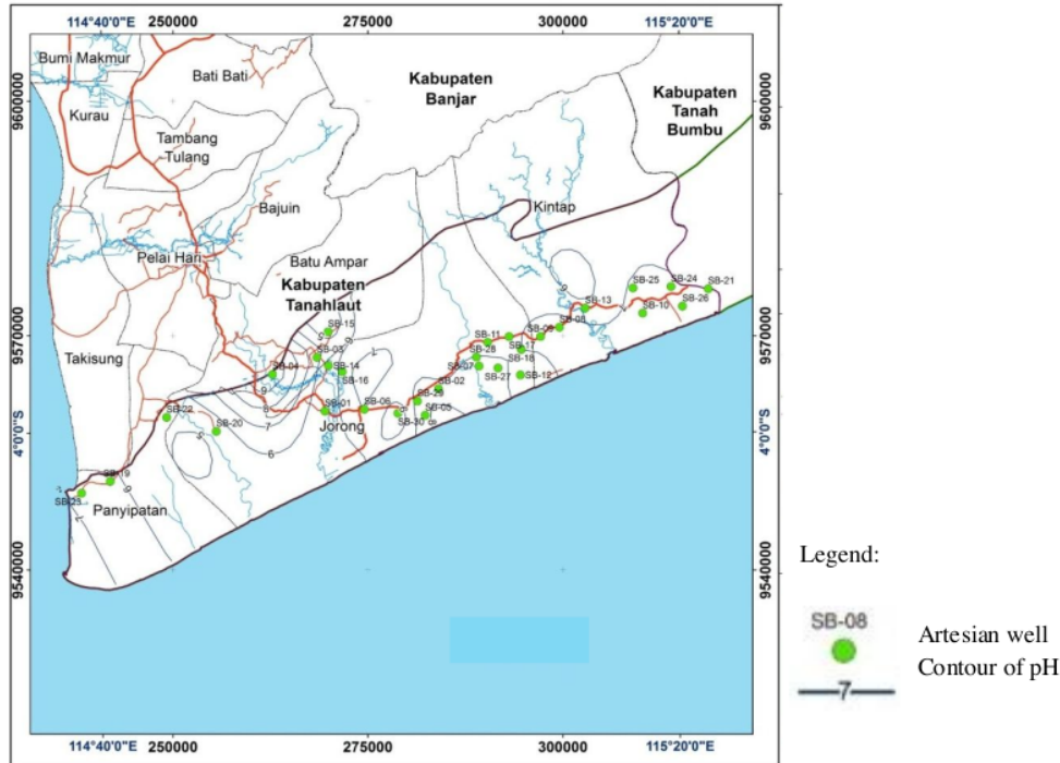
Figure 6. The distribution of pH in confined groundwater.
