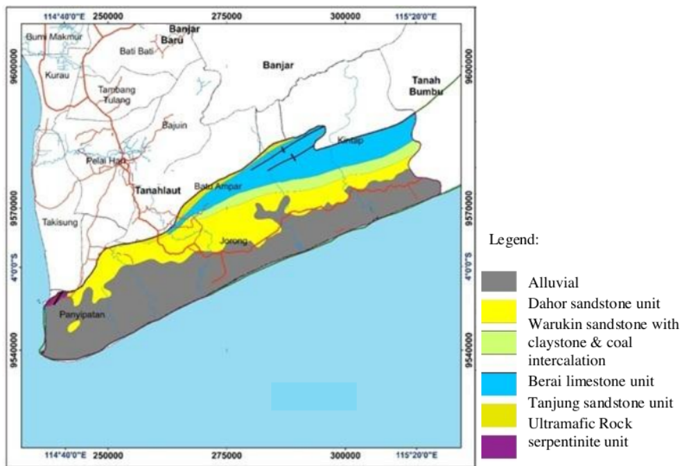
Figure 2. Geological map of research area.
