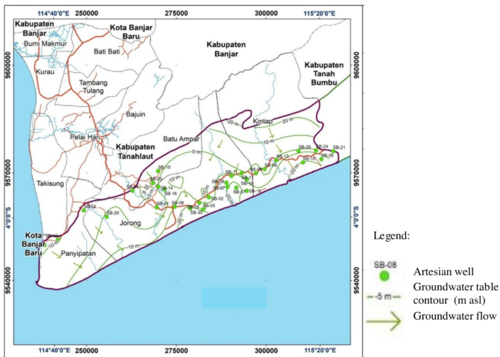
9 Figure 4. Groundwater table map of confined aquifer
