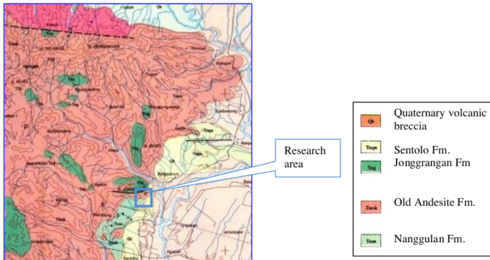
Figure 2. Geological map of research area [4].
