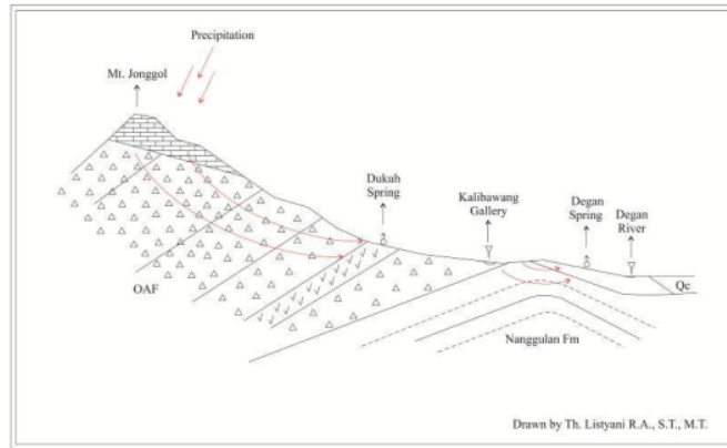
Figure 10. Isotopic hydrogeological setting of Banjararum area.
