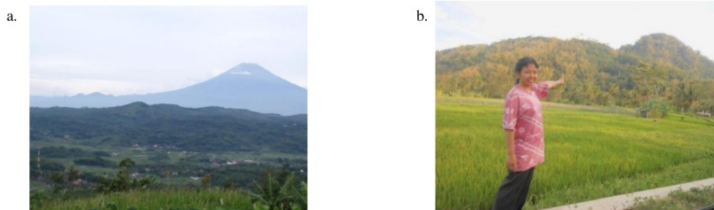
Figure 1. Morphology of Ungaran volcano.
