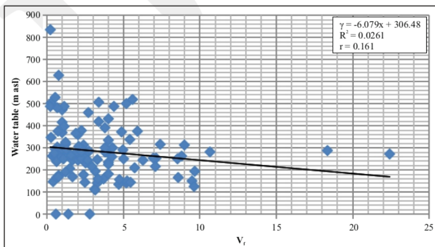
Figure 6. A correlation regression of V_r vs. water table, indicating a very weak or almost no relationship.
