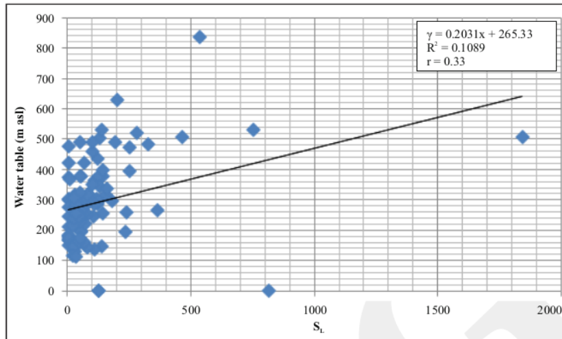
Figure 8. A correlation regression of stream gradient index ( S_t ) vs. water table, showing a bad or weak relationship.
