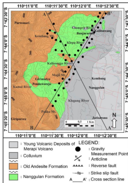
Fig.12 The gravity measurement by the point.
