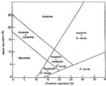
Gambar 1. Diagram Schaeffler (Honeycombe dan Badeshia, 1995)
