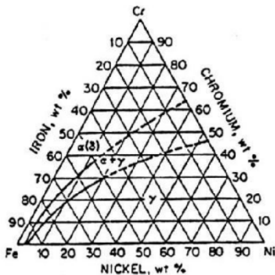
Gambar 2. Diagram fasa Fe-Cr-Ni (Leslie,1983)
