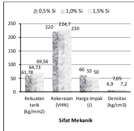
Gambar 5. Histogram sifat mekanik paduan Fe-7,5Al-5Mn-Si
