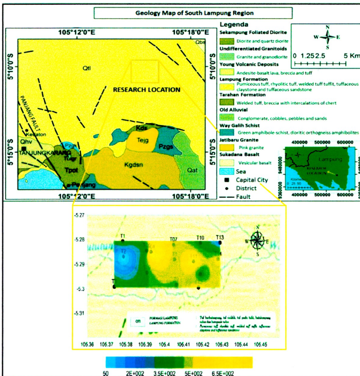
FIGURE 4: Interpretasi 2D menggunakan surfer in this study (Jati Agung Area of South Lampung, Indonesia). Source : Update from [13])
