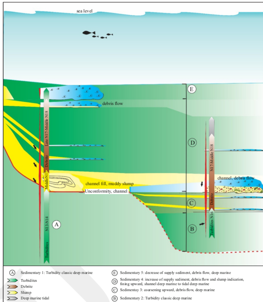
Figure 7. Illustration environment change of Rambatan Formation.
