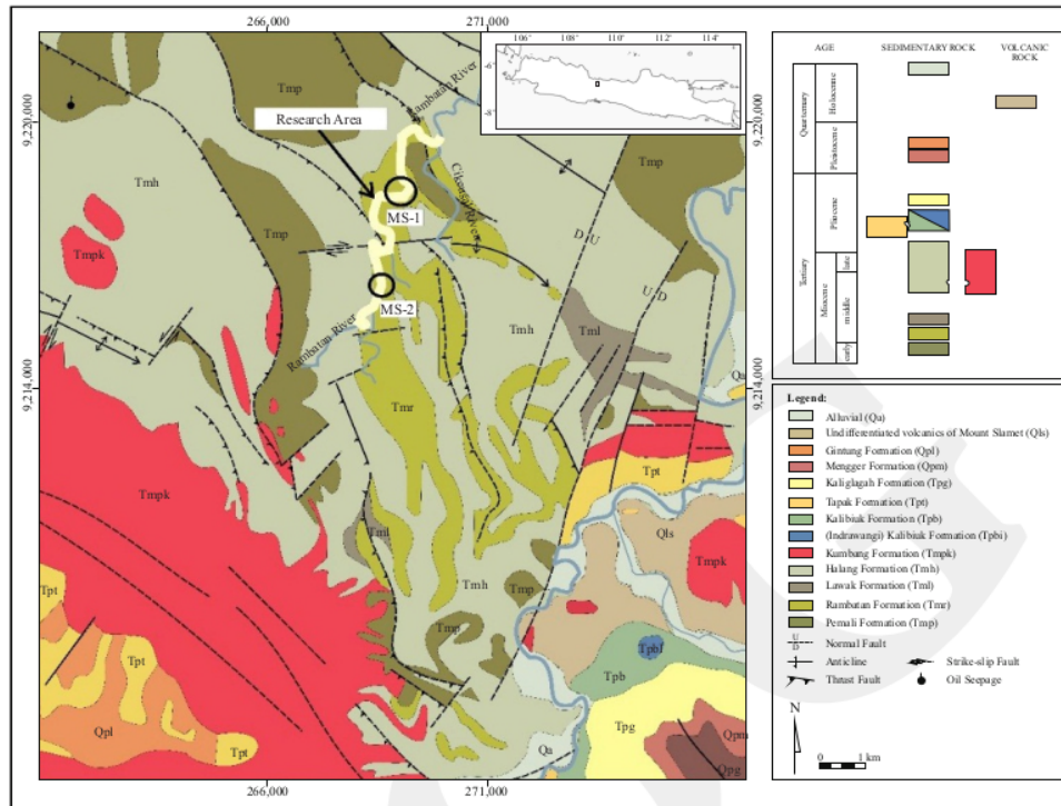
Figure 1. Regional map surrounding the researched area represented in white colour (source: Kastowo and Suwana, 1996).
